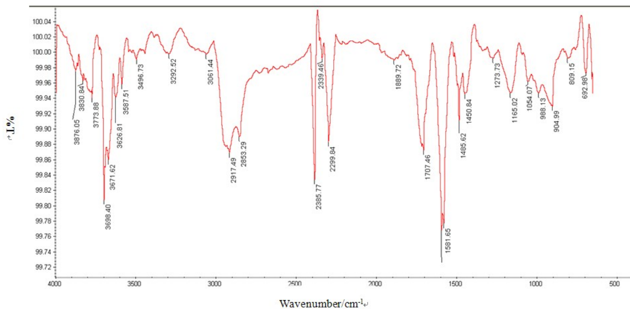
Figure S1 The FTIR spectra of the extracted component of DFS coal in THF
