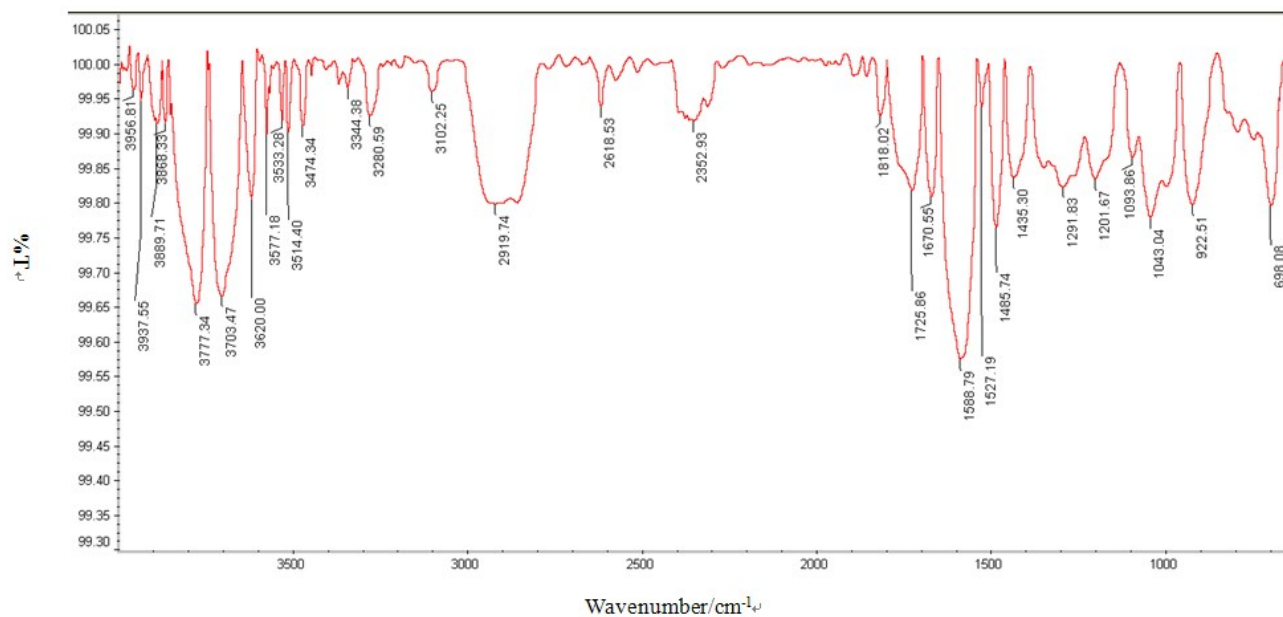
Figure S2 The FTIR spectra of the extracted component of DFS coal in DFS
