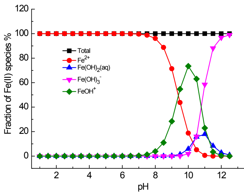
Fig.S1 Speciation of Fe(II) in water as a function of pH. (Calculated by employing Visual MINTEQ 3.0 software)
