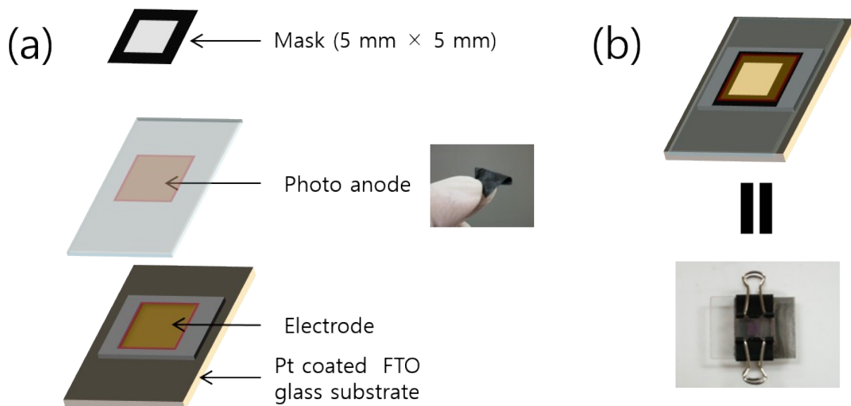
Figure S1. (a) Simple fabrication illustration of DDSC device with prepared photoanode, and (b) its digital photograph.
