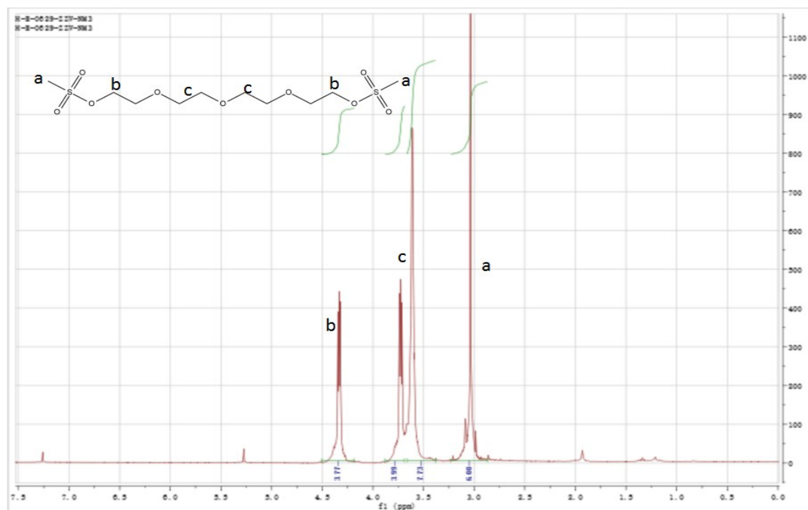
Figure S4 ^1\text{H-NMR} of precursor 10 to ionic liquid monomer M4
