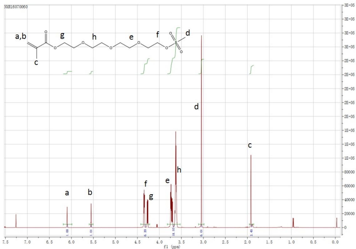
Figure S5 ^1\text{H-NMR} of precursor 11 to ionic liquid monomer M4
