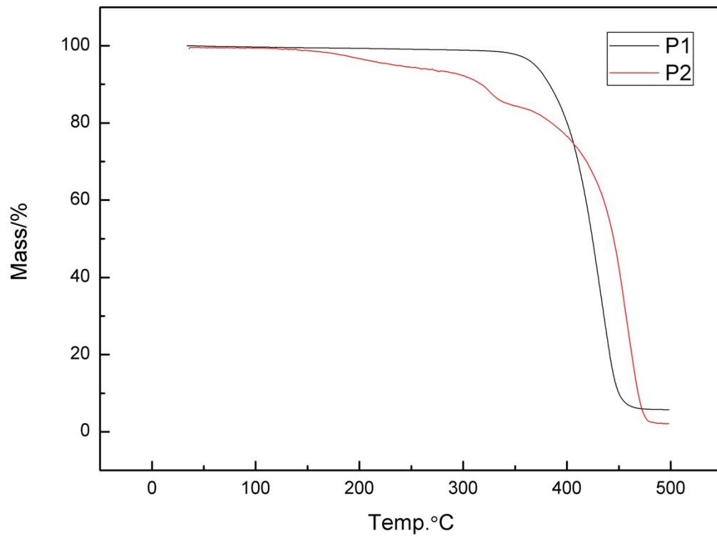
Figure S7 TGA graphic of P1 and P2
