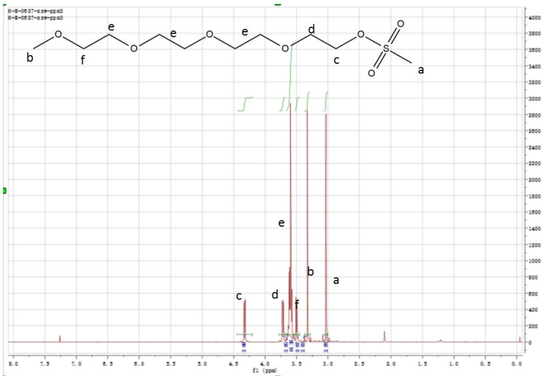
Figure S3 ^1\text{H-NMR} of precursor 7 to ionic liquid monomer M3
