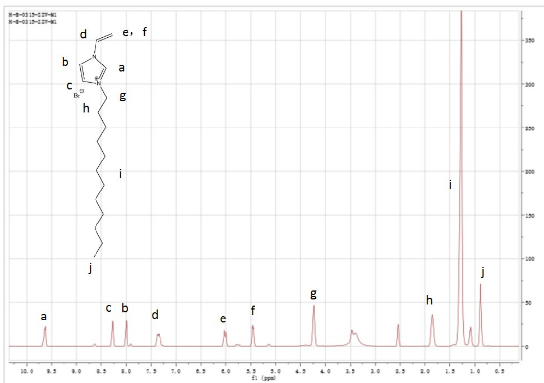
Figure S1 ^1\text{H-NMR} of precursor to ionic liquid monomer M1
