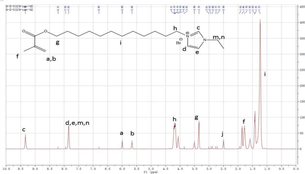
Figure S2 ^1\text{H-NMR} of precursor to ionic liquid monomer M2
