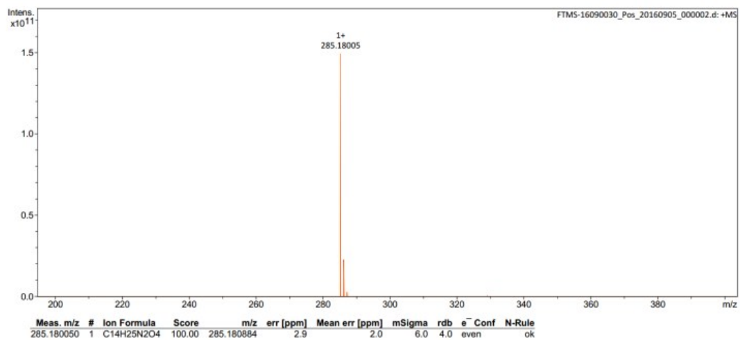
Figure S6 HR-Mass spectrum of cation of M3
