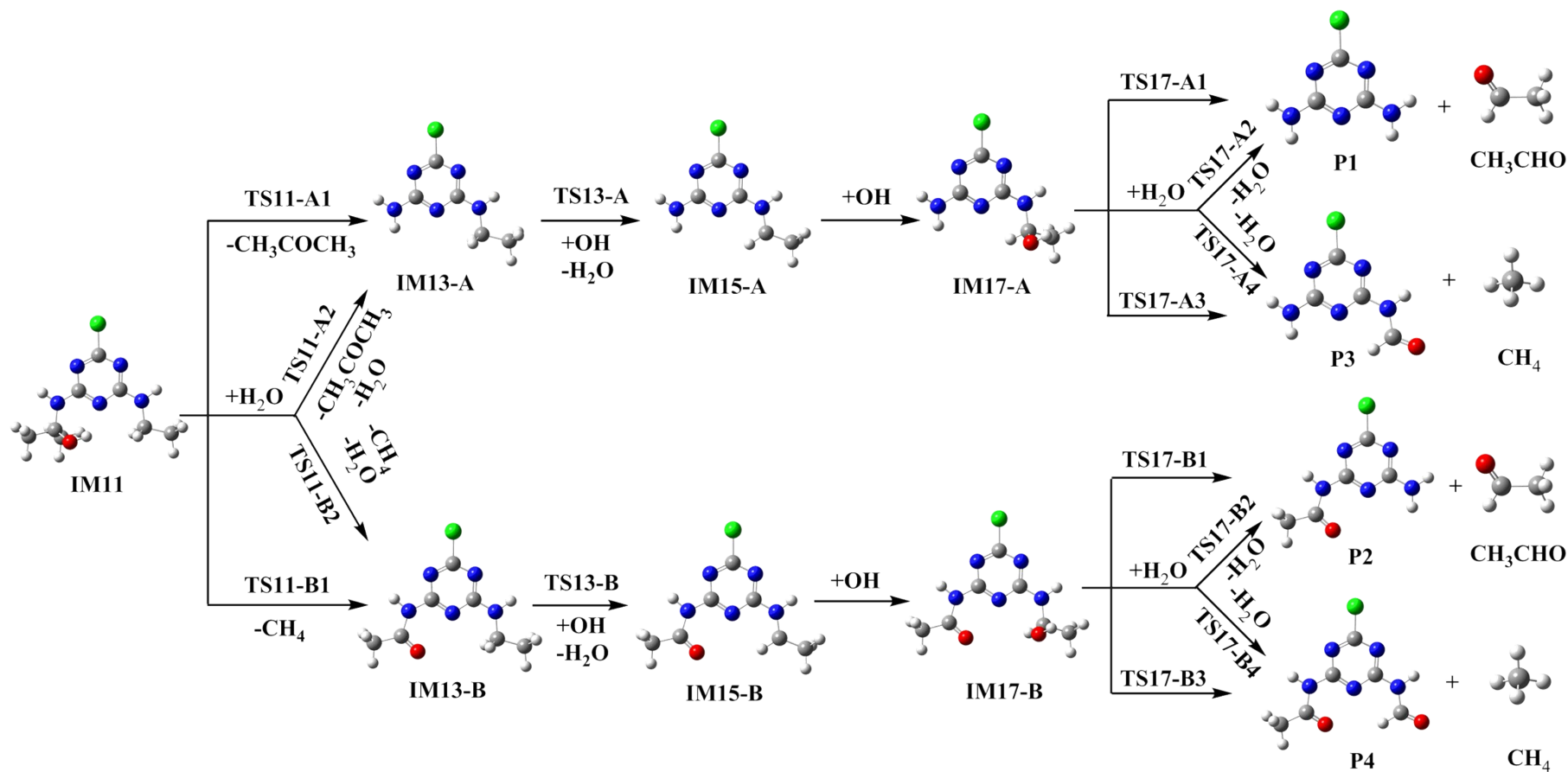
Figure S1 The dealkylation and alkyl oxidation process of IM11 in aqueous medium by Fenton oxidation technology
