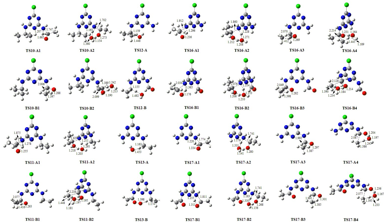
Figure S2 Optimized geometries for the transition states involved in the dealkylation and alkyl oxidation process. Distances are in angstroms
