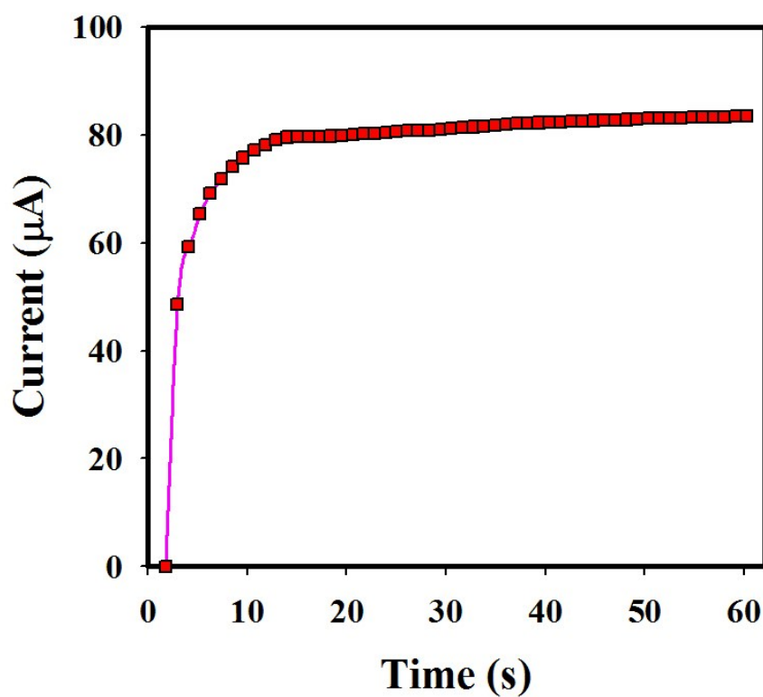
Fig. S1. Response time of uric acid detection by \text{Ce}_2\text{S}_3 -CNT NCs/GCE
