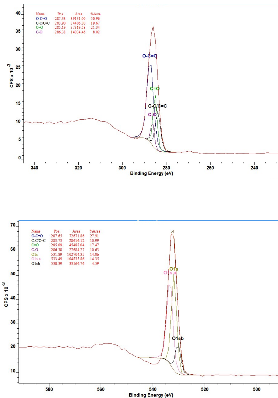
Supplementary Figure (S1) a) XPS of C1s of GO and the inset is the percentages of each deconvoluted peak regardless oxygen showing a ratio 1:4 between C=C/C-C peak and the other oxygenated peaks. B) XPS of O1s of GO and the inset is the total percentage of each peak.
