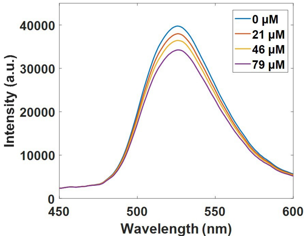
Supplementary Figure S1. Fluorescence spectra of HPTS (10 mM, pH 6.5, 22°C) in deionized water with increasing concentrations of BPA (0-79 μM). Spectra were measured at 90° from an incident 460 nm LED light source.
