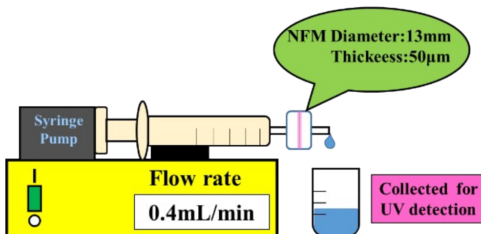
Figure S1 Experimental set-up for the investigation of continuous catalytic hydrogenation of 4-NA using POM/PLLA-Ag NFMs
