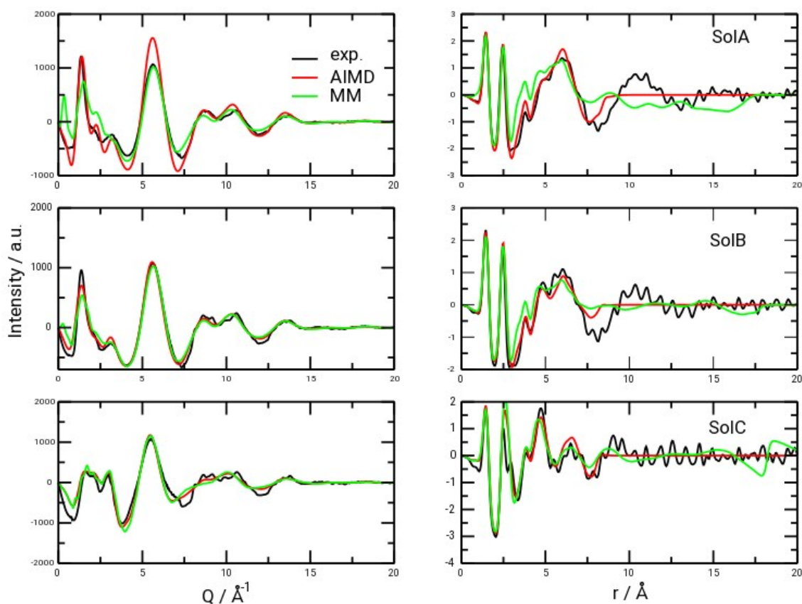
Fig. 1 : Left side: theoretical and measured structure function. Right side: theoretical and measured radial distribution function. Moving from top to bottom the water concentration increases.
