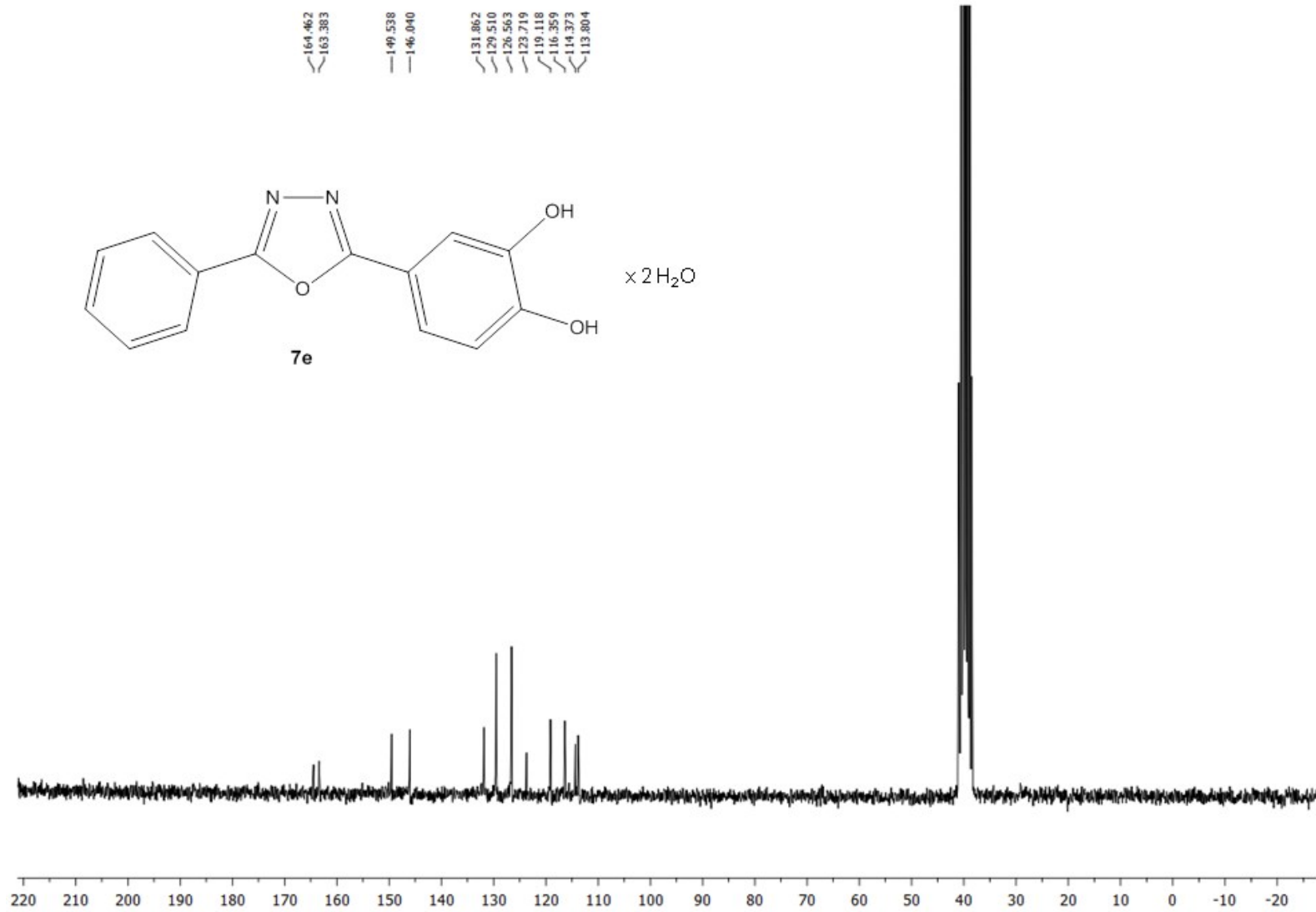
Figure S26. 13 C NMR spectrum of 7e in DMSO-d 6 (50 MHz).
