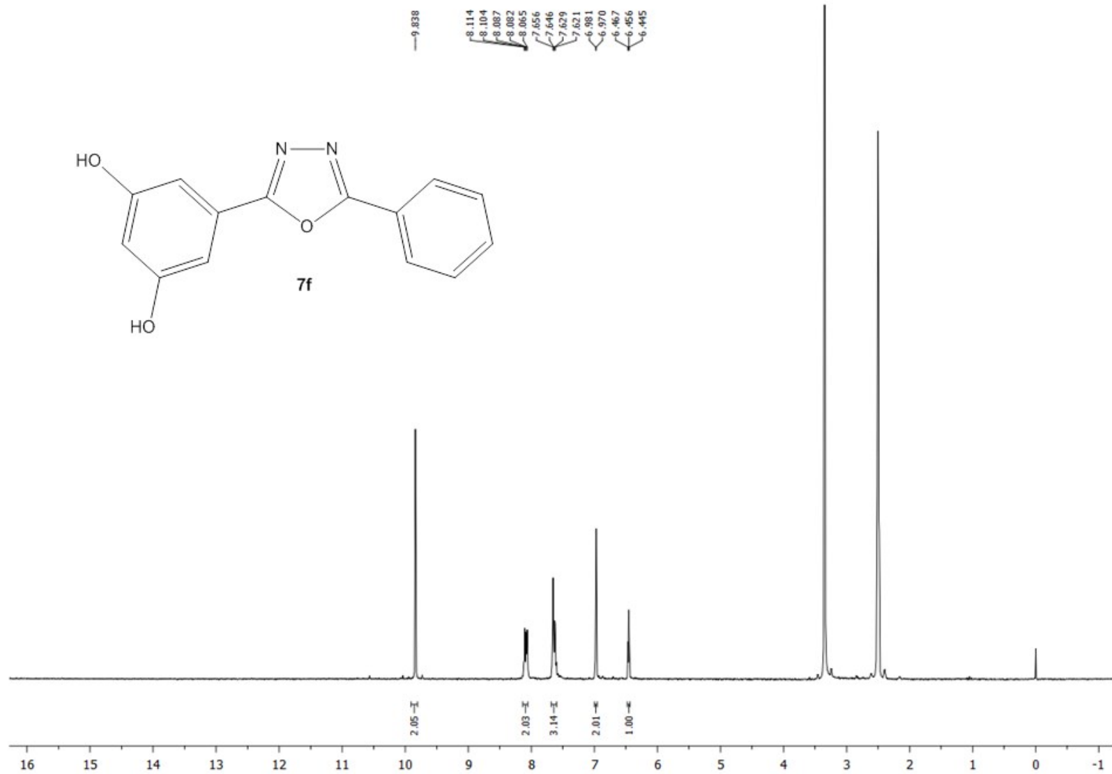
Figure S27. ^1\text{H} NMR spectrum of 7f in \text{DMSO-d}_6 (200 MHz).
