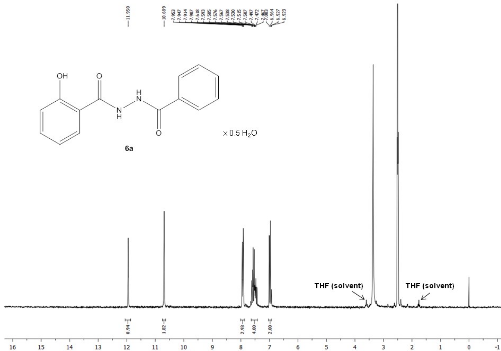
Figure S1. 1 H NMR spectrum of 6a in DMSO-d 6 (200 MHz).
