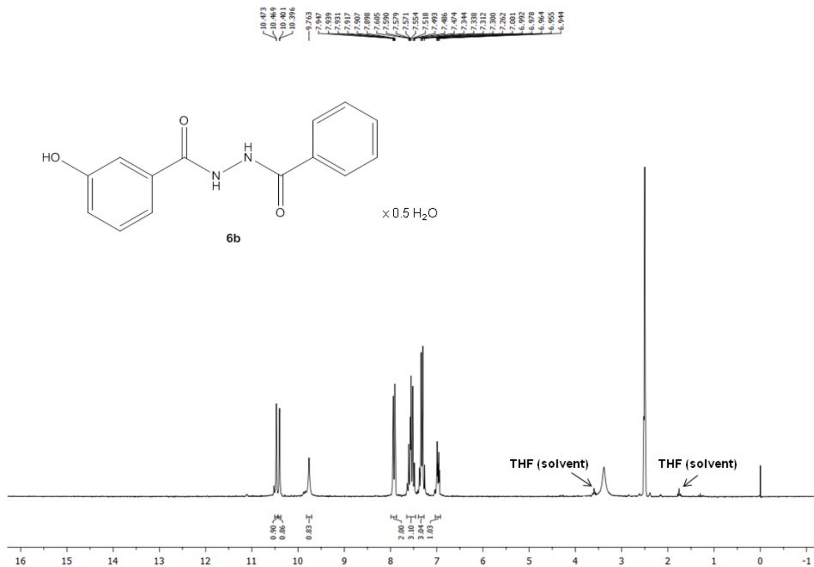
Figure S3. ^1\text{H} NMR spectrum of 6b in \text{DMSO-d}_6 (200 MHz).
