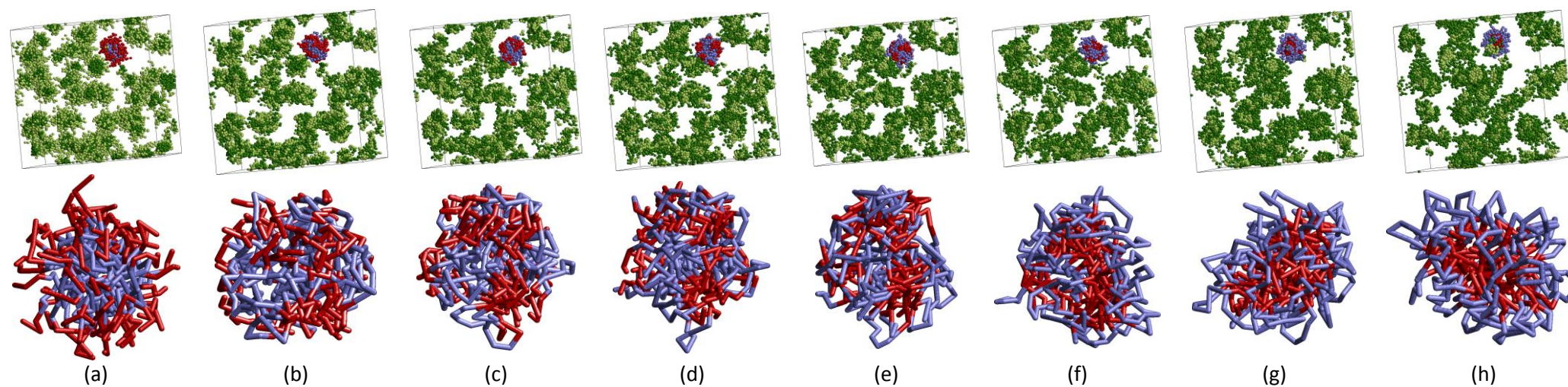
5 vol% A_3B_6A_3 surfactants co-polymers in solvent S_1 changed to solvent S_2 . (a) 0, (b) 370, (c) 750, (d) 1100, (e) 1500, (f) 2410, (g) 4000, and (h) 16000 time steps. Top row is the full box, bottom row is one example micelle.
