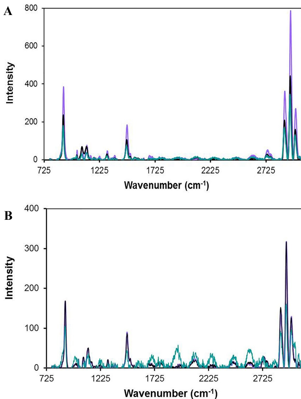
Figure S1. Raman spectra of a) freshly prepared and b) aged 30% zein in 70% ethanol (purple), 80% ethanol (black), 90% ethanol (green).
