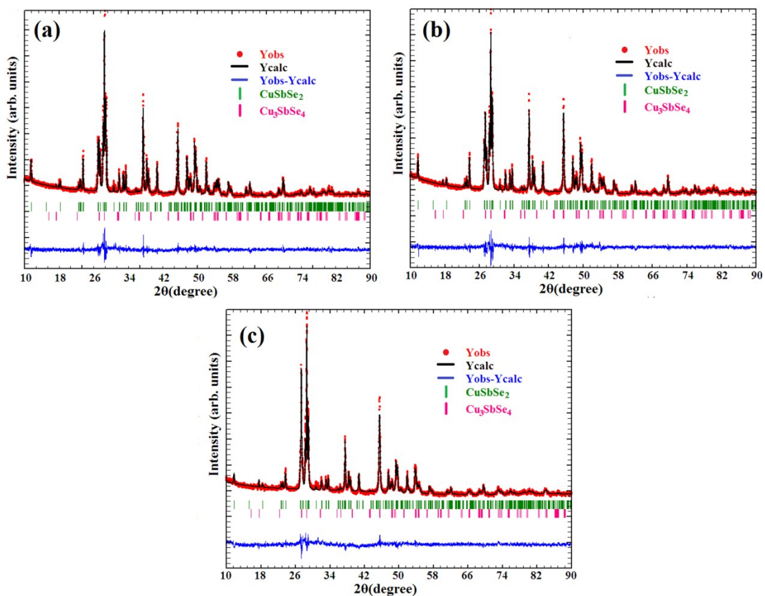
Fig. S1. Rietveld refinement using X-ray diffraction data for \text{CuSbSe}_2 bulk sample (a) 2\theta = 1 ; (b) 9 - 1 ; (c) 8 - 2 .
