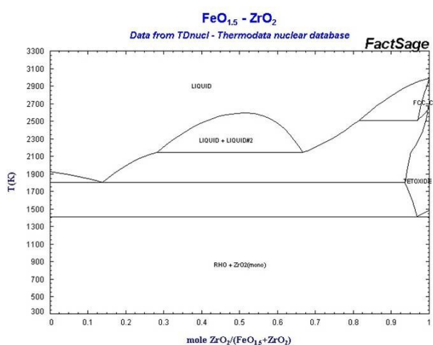
Fig S1. The phase diagram of \text{ZrO}_2 - \text{Fe}_2\text{O}_3 .
