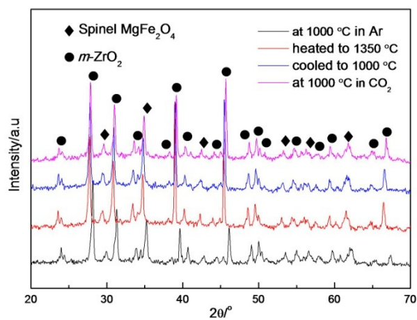
Fig S2. The in-situ high temperature XRD patterns of the 30 wt % \text{MgFe}_2\text{O}_4 / \text{ZrO}_2 .
