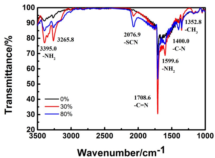
Fig. S1 Fourier transform infrared spectra of FAPbI 3 perovskite films with and without SCN.
