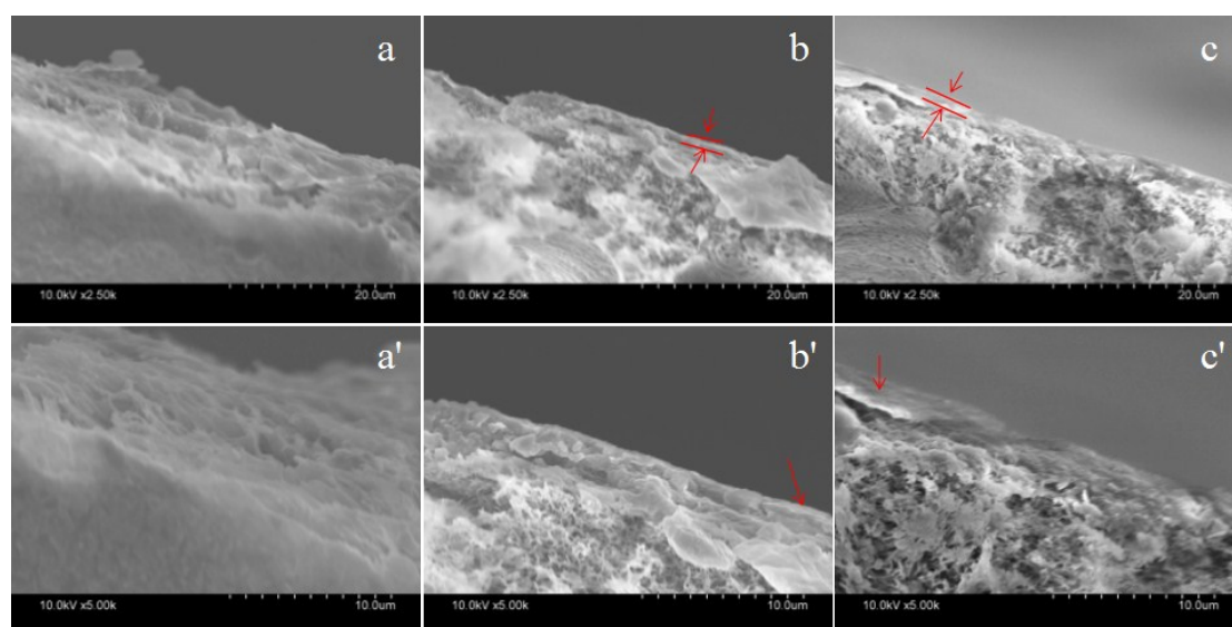
Fig. S1 Cross-section SEM images of original (a,a'), PA-g-PEG/TAEA (b,b') and PA-g-PEG/SMZ (c,c') membranes (a-c 2500 \times , a'-c' 5000 \times ).
