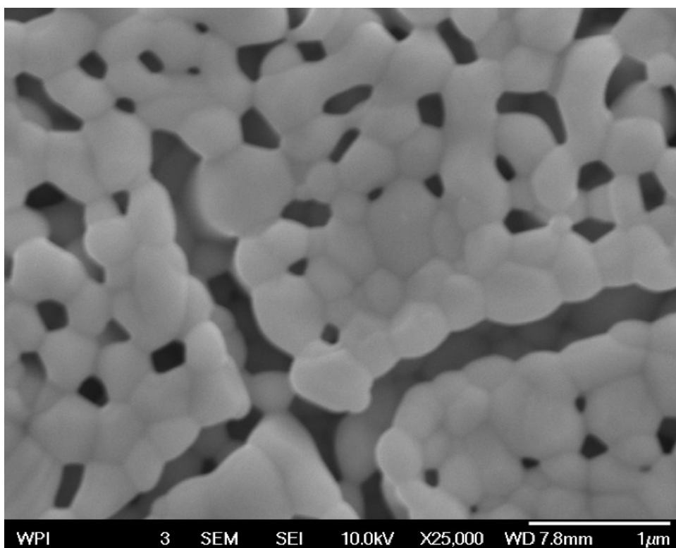
Supplementary Figure S1. SEM micrograph of BiVO 4 film on quartz substrate.
