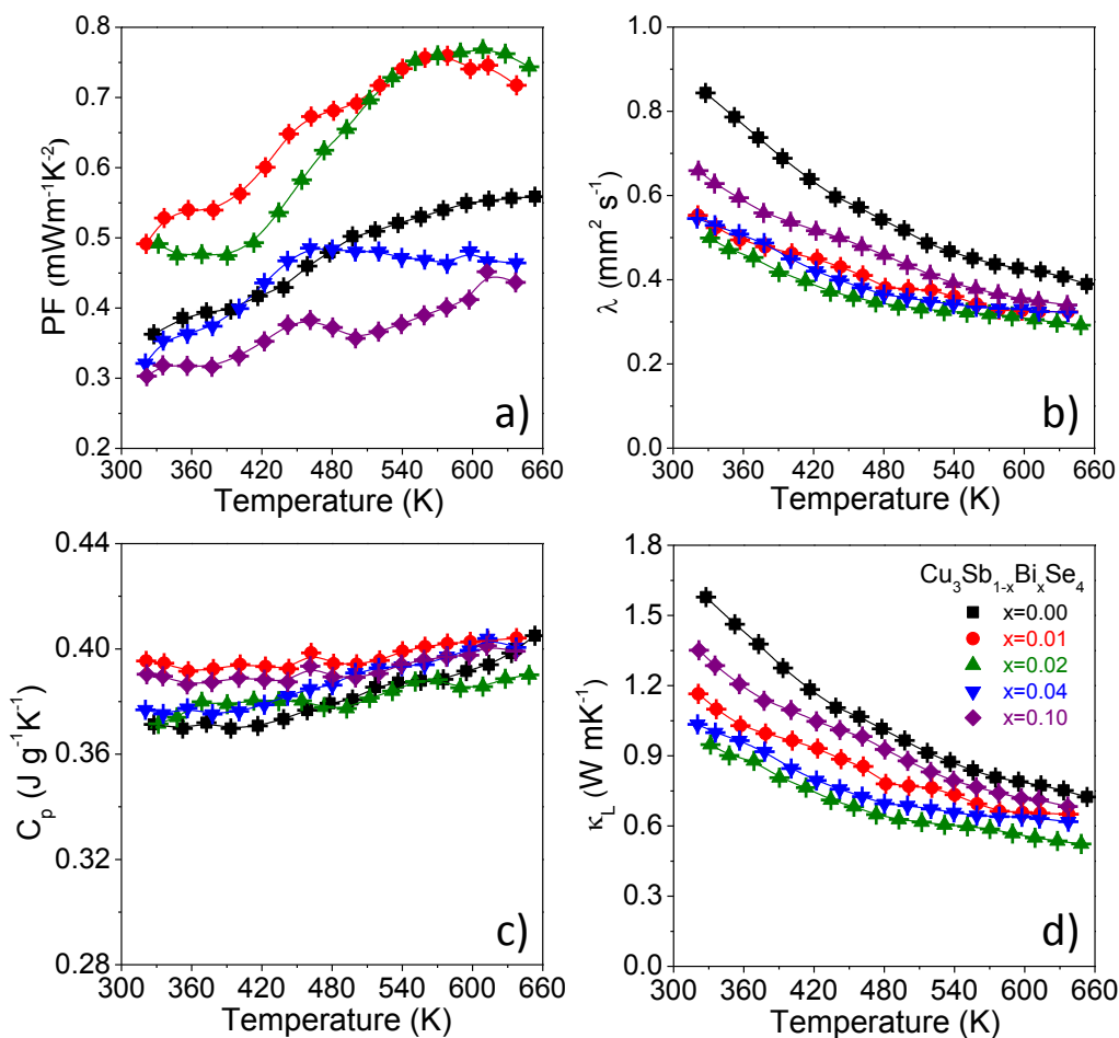
Figure S19. Temperature dependence of (a) power factor (PF), (b) thermal diffusivity ( \lambda ), (c) specific heat ( C_p ), and (d) lattice thermal conductivities ( \kappa_L ) of \text{Cu}_3\text{Sb}_{1-x}\text{Bi}_x\text{Se}_4 ( x=0.01, 0.02, 0.04 and 0.10 ).
