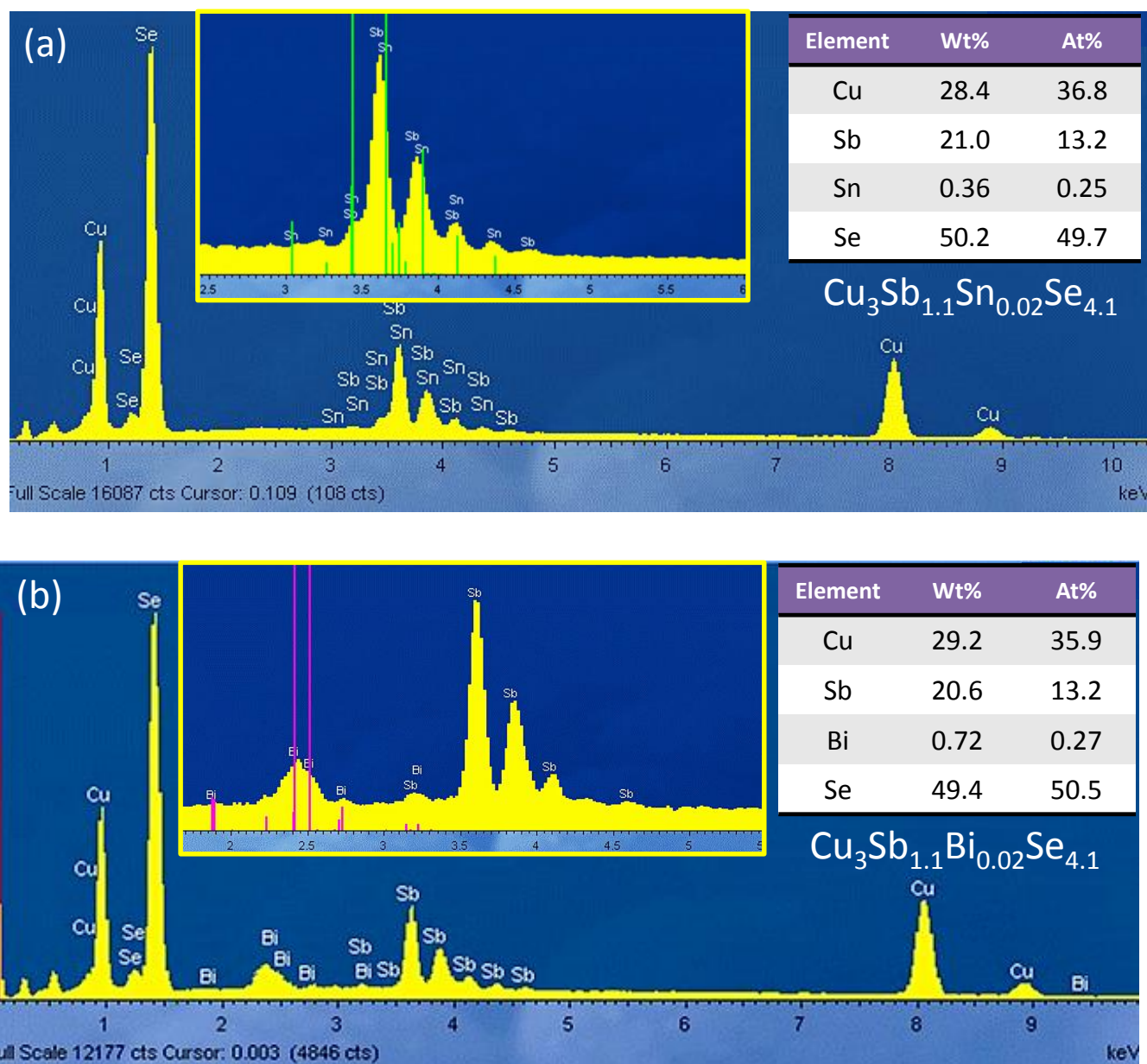
Figure S12. Representative SEM-EDX spectra of Sn-CASe and Bi-CASe consolidated materials.
