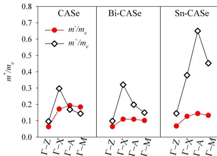
Figure S22. Effective masses for electrons ( m^- ) and holes ( m^+ ) calculated from DFT for CAs 2 Se, Bi-CAs 2 Se and Sn-CAs 2 Se
