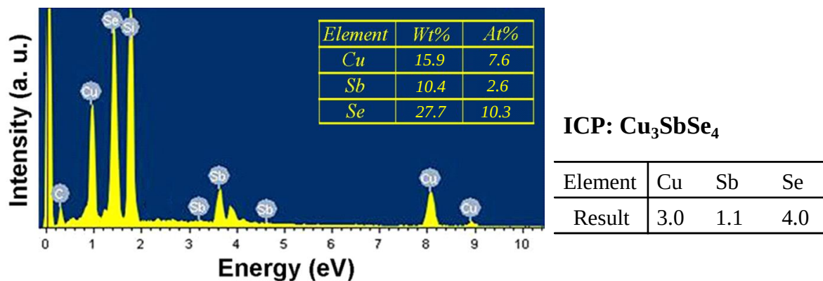
Figure S4. Left: EDX spectrum of CSe NCs and quantitative analysis of the as-synthesized CSe NCs showing a composition consistent with stoichiometric \text{Cu}_3\text{SbSe}_4 . Right: Results of the ICP analysis of CSe NCs showing a composition of \text{Cu}_{3.0}\text{Sb}_{1.1}\text{Se}_{4.0} .
