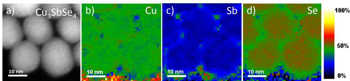
Figure S5. (a) HAADF-STEM image of CSe NCs. (b-d) relative atomic composition of Sb, Cu and Se.
