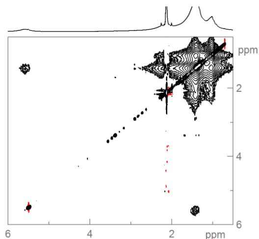
Figure S13. NOESY spectrum of CAs synthesized with OA.
