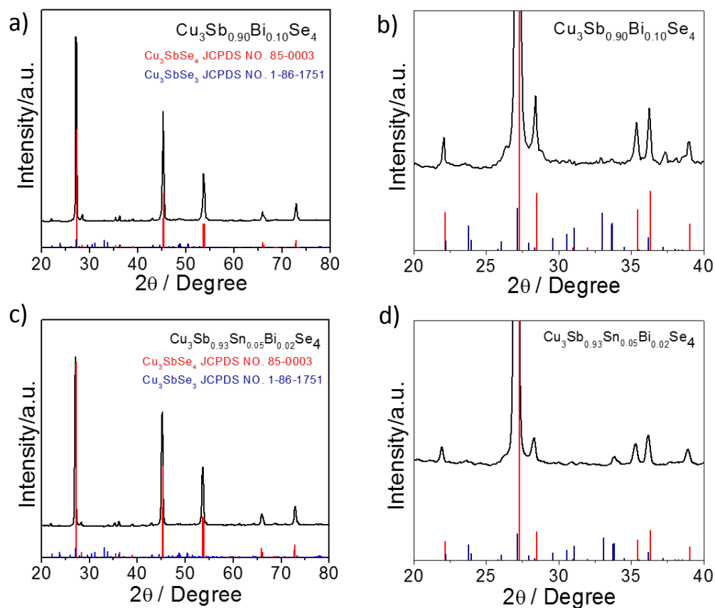
Figure S3. XRD patterns (a,c) and detail of the (112) peaks between 20^\circ and 40^\circ 2\theta values (b,d) of \text{Cu}_3\text{Sb}_{0.90}\text{Bi}_{0.10}\text{Se}_4 (a,b) and \text{Cu}_3\text{Sb}_{0.93}\text{Sn}_{0.05}\text{Bi}_{0.02}\text{Se}_4 (c,d) pellets. Red vertical lines correspond to the reference literature data for \text{Cu}_3\text{SbSe}_4 , JCPDS NO. 85-0003. Blue vertical lines correspond to \text{Cu}_3\text{SbSe}_3 , JCPDS NO. 1-86-1751.
