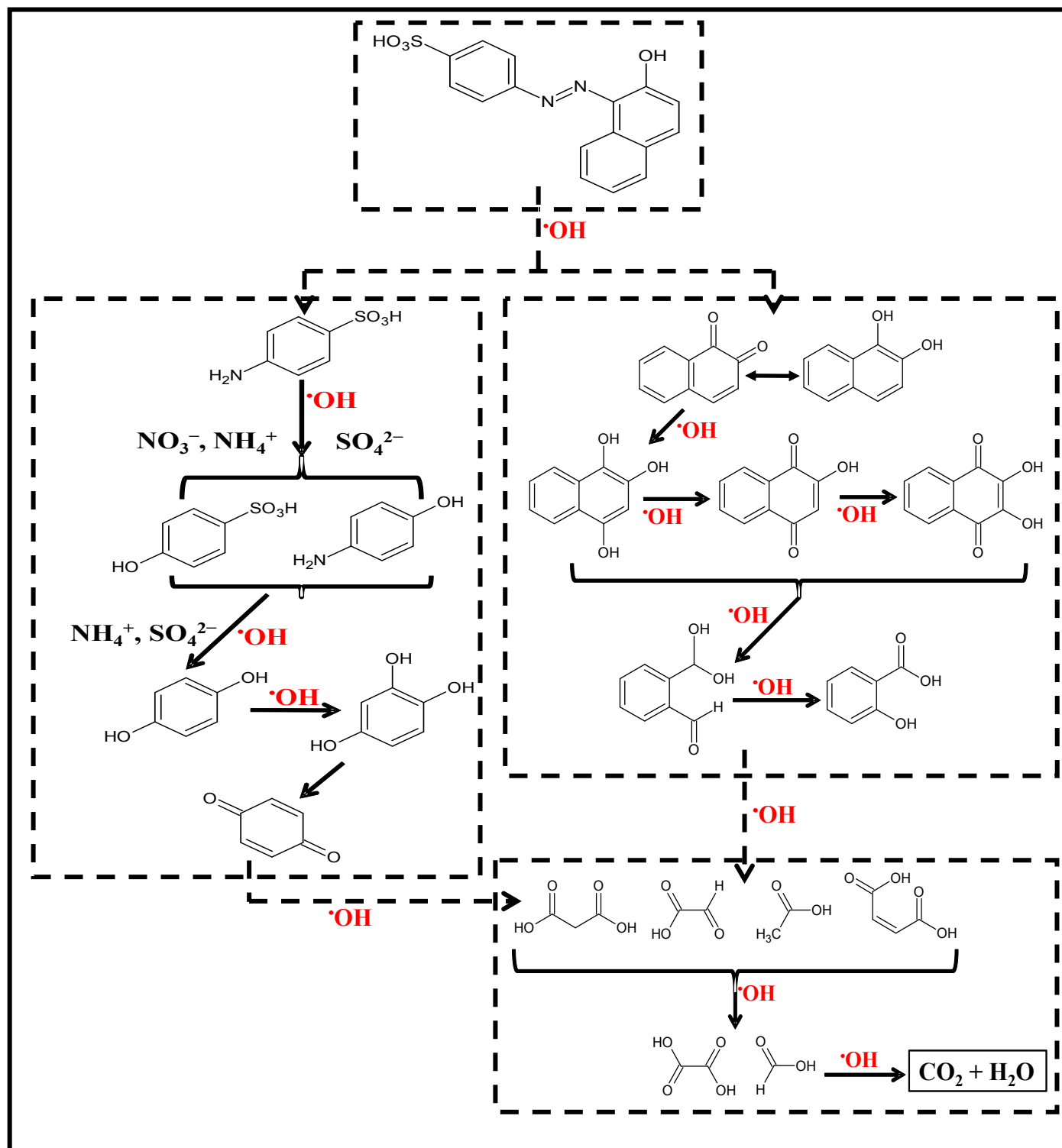
Figure S1. Reaction mechanism for complete degradation of AO7 by \cdot\text{OH}
