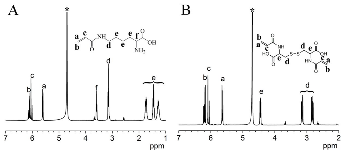
Fig. S1 ^1\text{H} NMR spectra of (A) LysAAm and (B) BACystine in \text{D}_2\text{O}
