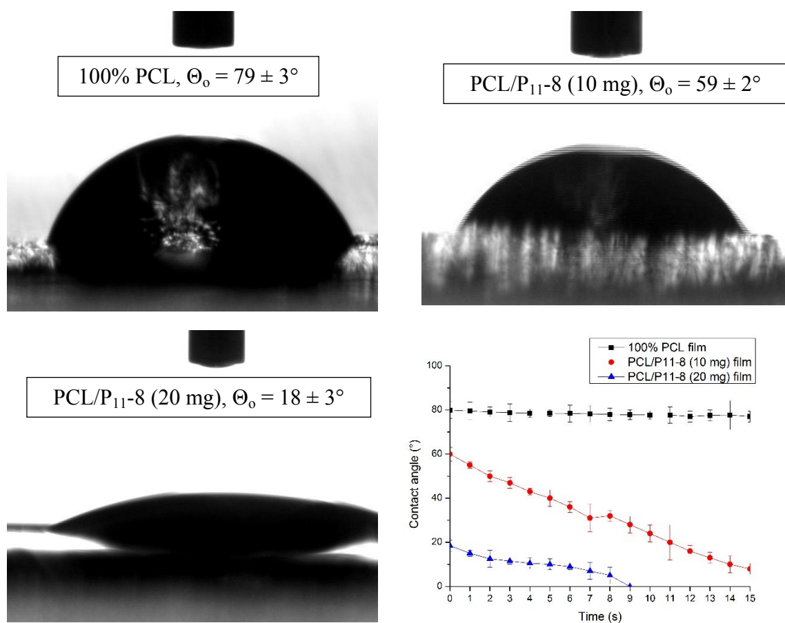
Figure S1. Contact angle of water on PCL and PCL/P 11 -8 cast films showing enhanced hydrophilicity with increased peptide concentration.
