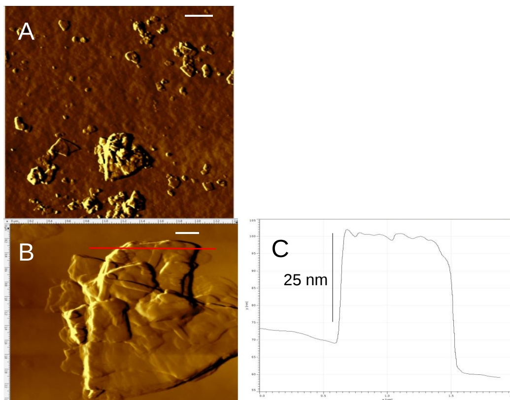
Fig. S1. (A,B) Contact mode AFM of GO dried on cleaned silicon surface (scale bar 1 μm in A and 0.2 μm in B). (C) Height line profile of red line shown in (B).
