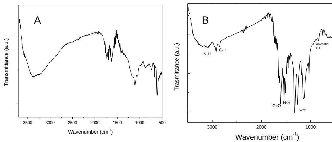
Fig. S2. FTIR spectrum of (A) GO and (B) GO-NOP1
