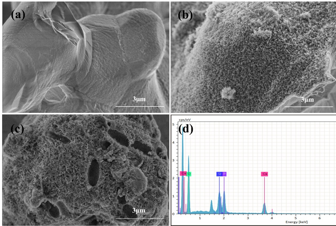
Supplementary Fig. 2 SEM images and EDS analysis for SPS powders soaked in SBF for 0 (a), 1 (b) and 7 days (c, d).
