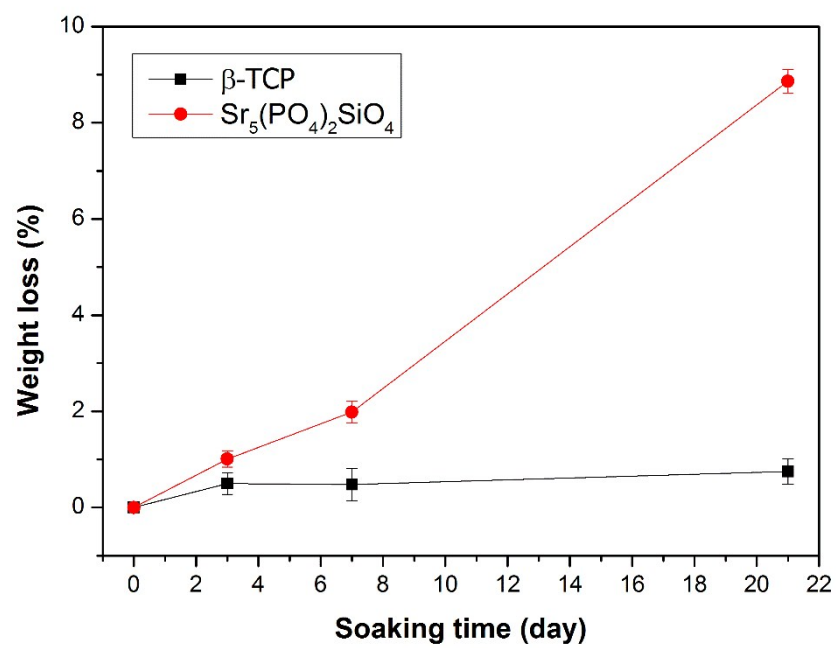
Supplementary Fig. 3 The weight loss of \beta -TCP and SPS scaffolds in Tris-HCl solution.
