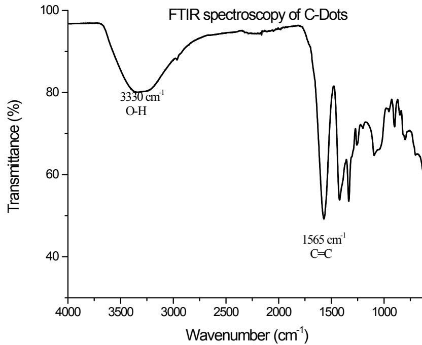
Figure SI 1. Fourier transform infrared spectroscopy of C-dots.
