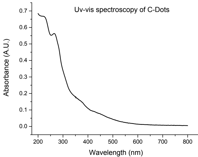
Figure SI 2. Uv-vis spectroscopy of C-dots.
