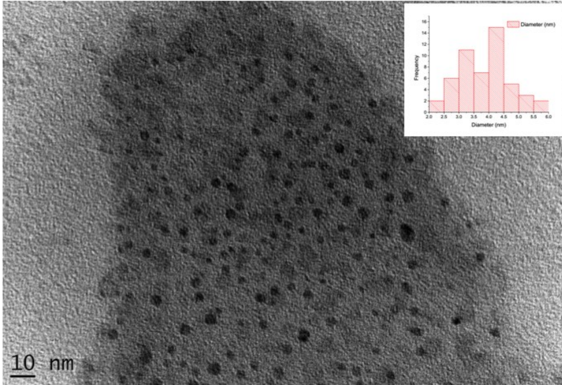
Figure SI 3. Transmission electron spectroscopy of C-dots, inset is the size distributions of the particles.
