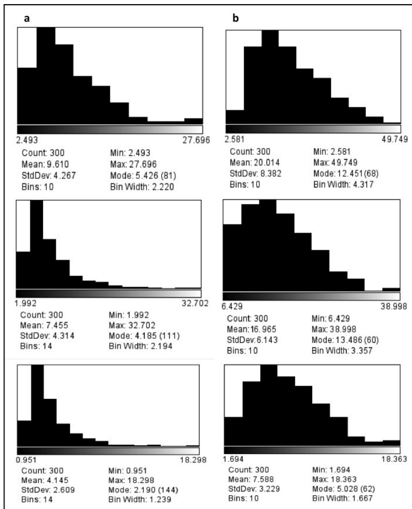
Figure S1. Porosity analysis by Image-J for silk and silk/PEO blends. a. Top to bottom: 13, 14 and 15% silk microtubes; b. Top to bottom: blends of PEO 1% and silk 13, 14 and 15% microtubes. Number of pores like a function of pore size (micrometers) for 300 measures is showed for each system. Mean values, maximum, minimal and mode, as well as Standard Deviation are indicated.
