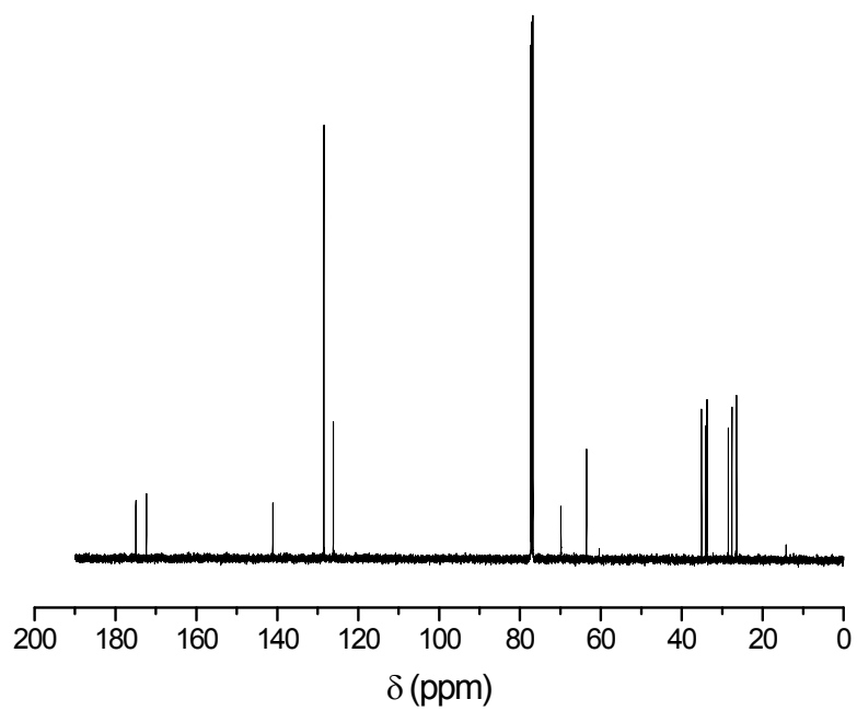
Figure S7. 13 C NMR of \gamma -Phenylbutyrate- \epsilon -Caprolactone
