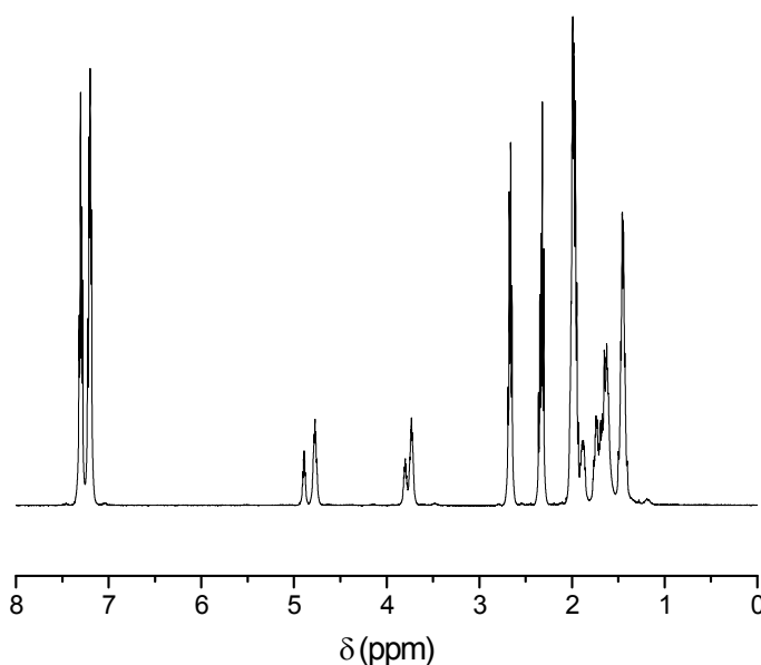
Figure S1. 1 H NMR of 4-hydroxycyclohexyl-4-phenylbutanoate
