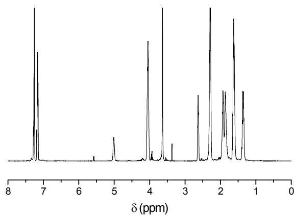
Figure S9. ^1\text{H} NMR of P1
