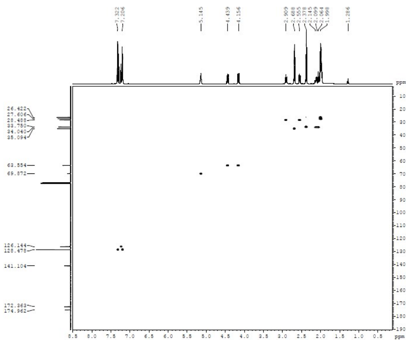
Figure S8. HSQC of \gamma -Phenylbutyrate- \epsilon -Caprolactone
