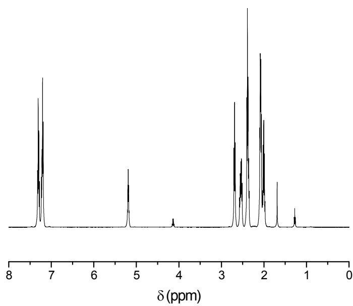
Figure S3. ^1\text{H} NMR of 4-oxocyclohexyl-4-phenylbutanoate
