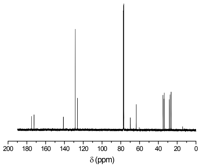
Figure S4. ^{13}\text{C} NMR of 4-oxocyclohexyl-4-phenylbutanoate
