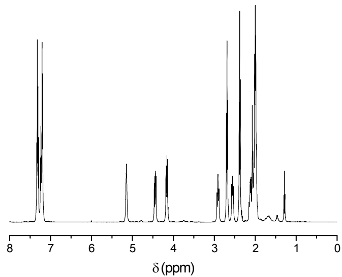
Figure S6. 1 H NMR of \gamma -Phenylbutyrate- \epsilon -Caprolactone
