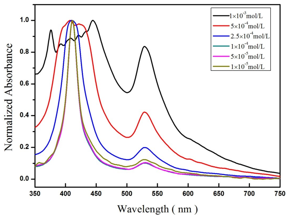
Figure S1. Concentration-dependent UV-Vis spectra of DETPP-P-Co ( \text{CH}_2\text{Cl}_2 , 298 K).
