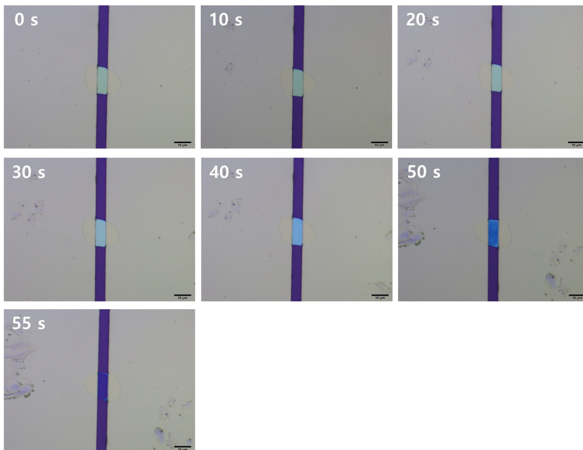
Figure S11. Optical microscope images of the fabricated BP FET as a function of plasma treatment time
