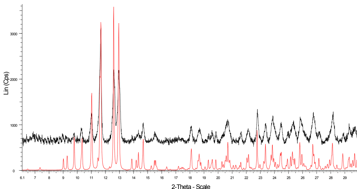
XRPD of (1) : theoretical (red) and experimental (black)
