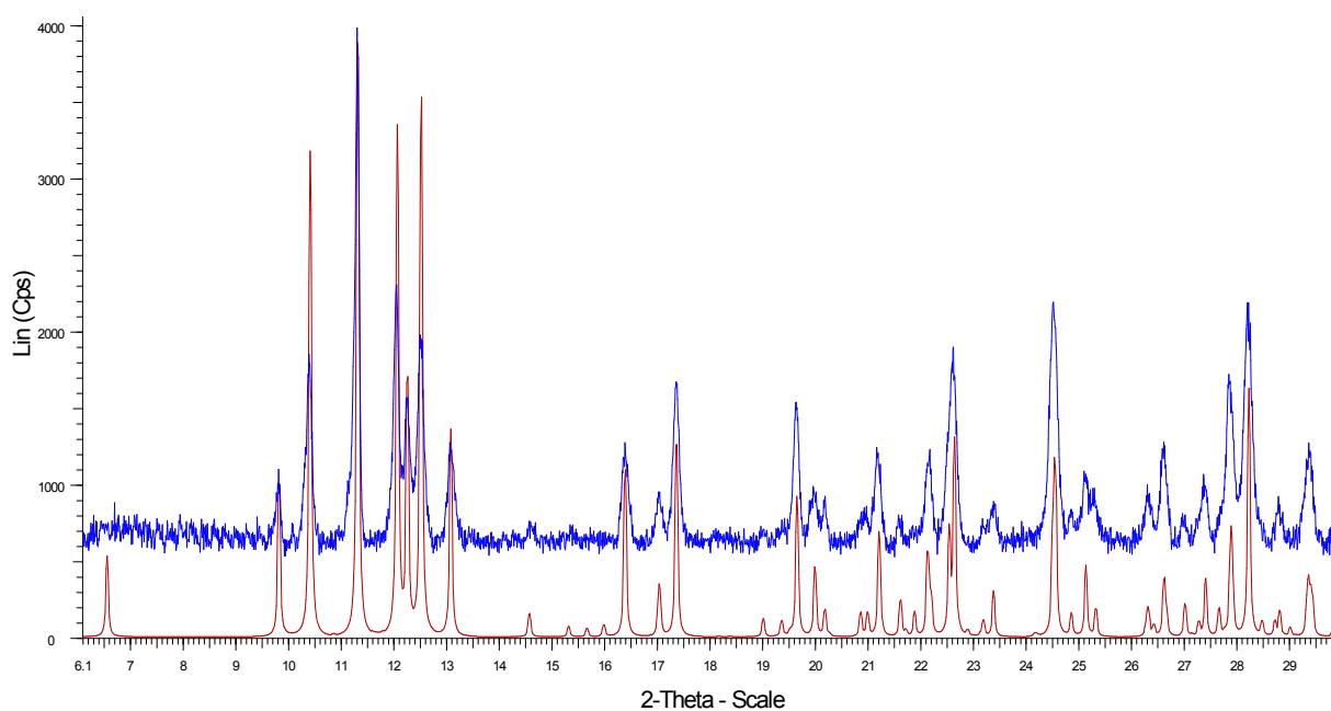
XRPD of (2) : theoretical (dark-red) and experimental (blue)
