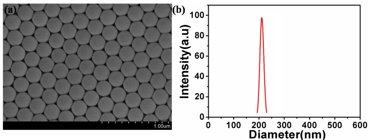
Figure S1 The characterization of as prepared latex spheres' diameter (a) and size distribution (b), whose PDI is lower than 0.005.
