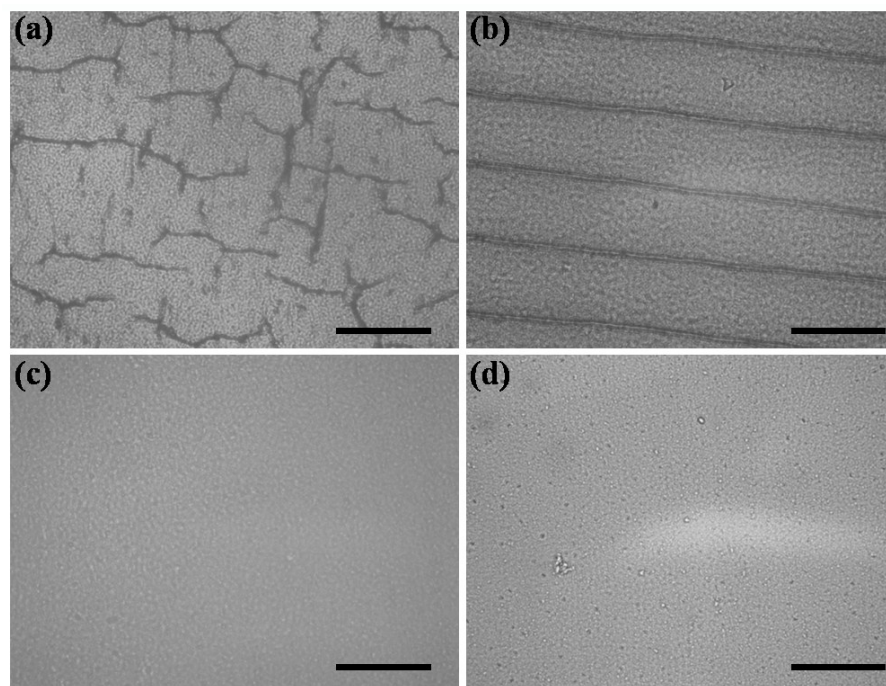
Figure S2 The optical microscopy images of as prepared PCs films. Mass ratios of zirconium ammonium carbonate to polymer latex spheres were 0:100, 0.5:100, 1:100 and 2:100 (a-d), scale bar is 500 μm.
