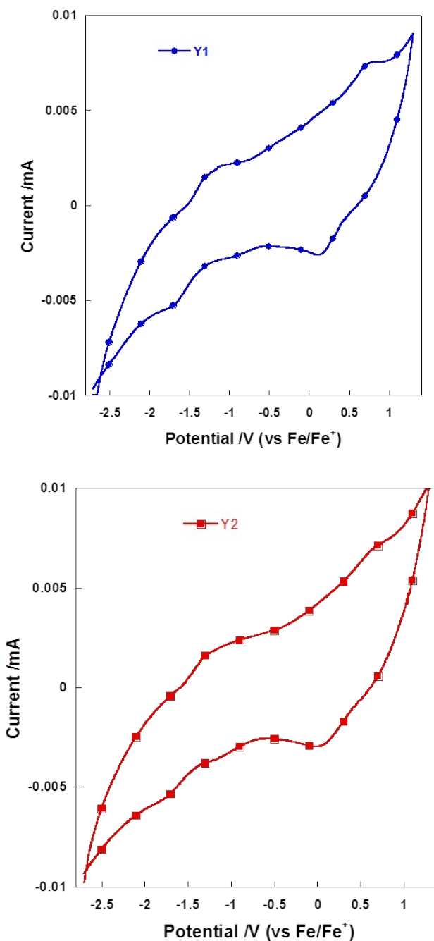
Figure S1. CV curves of iridium complexes Y1 and Y2 in THF.
