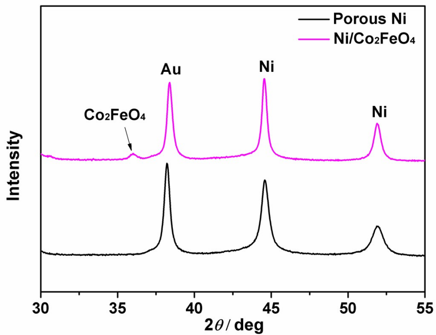
Fig. S2 XRD patterns of porous uncoated Ni and Ni-supported Co 3-x Fe x O 4 samples.
