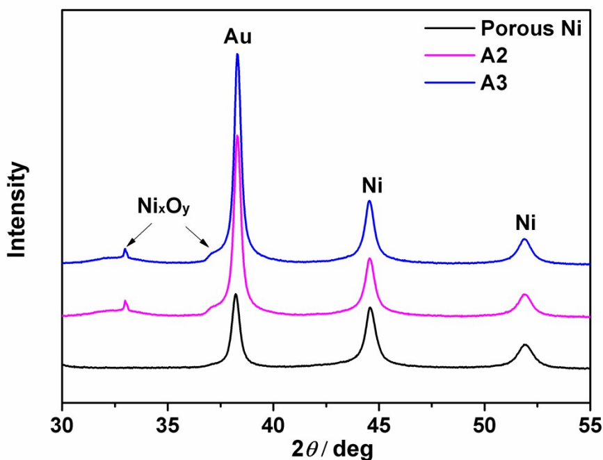
Fig. S1 XRD patterns of porous uncoated Ni, and A2 and A3 composite samples.
