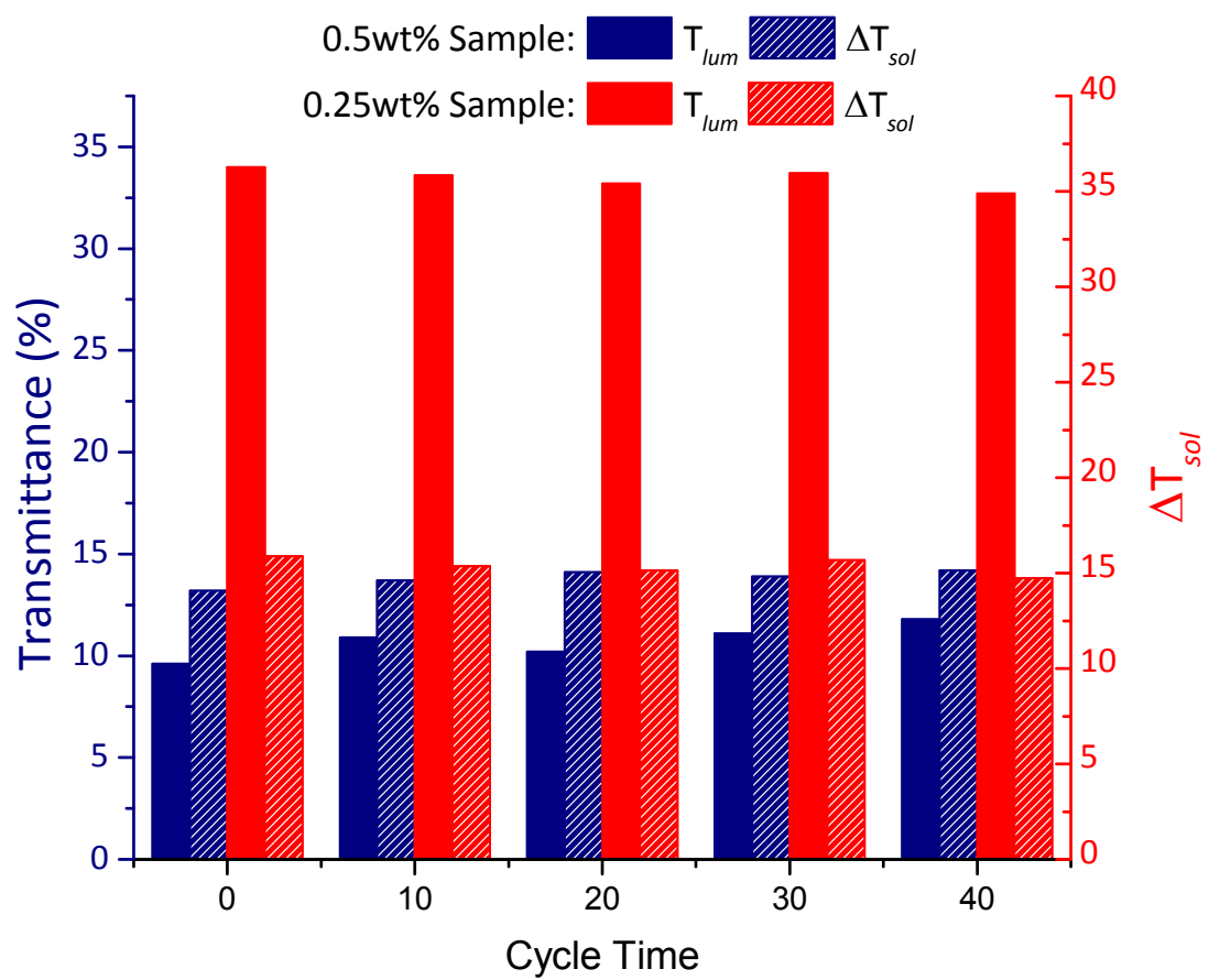
Figure S3. Cycling test for both 0.5wt% and 0.25wt% samples indicate minimum variations in their transmittance and solar modulation after 40 cycles.
