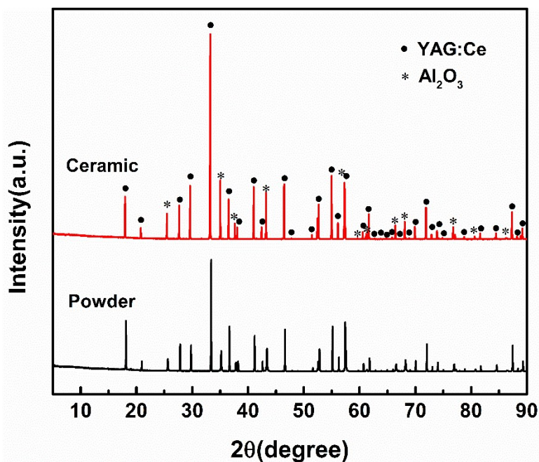
Fig. S1. The XRD patterns of the as-mixed powders and the sintered composite phosphor ceramic.
