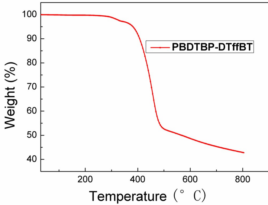
Fig.S1 TGA plot of PBDTBP-DTffBT
