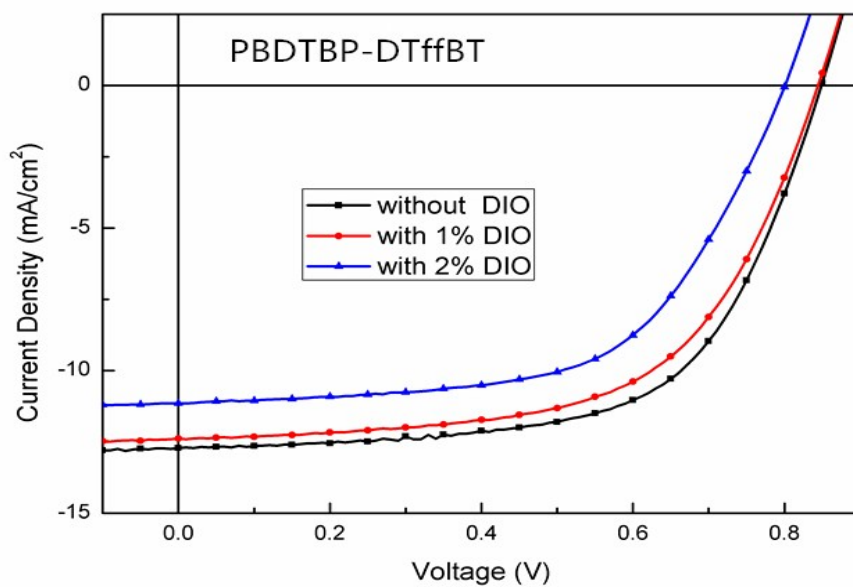
Fig. S4 .The J-V curves of PSCs with different weight ratios DIO
