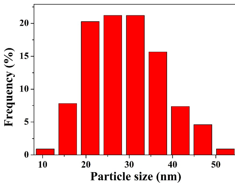
Figure S2. Particle size distribution of pure NZCF particles.
