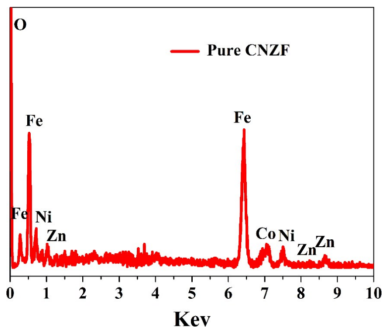
Figure S1. EDS spectrum of the pure CNZF
