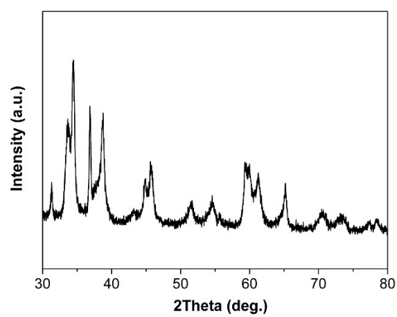
Fig. S1 XRD pattern of the precursor.
