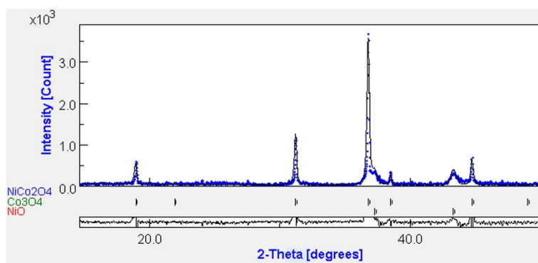
Fig. S2 XRD pattern and Rietveld analysis pattern of \text{NiCo}_2\text{O}_4/\text{Co}_3\text{O}_4/\text{NiO} .
