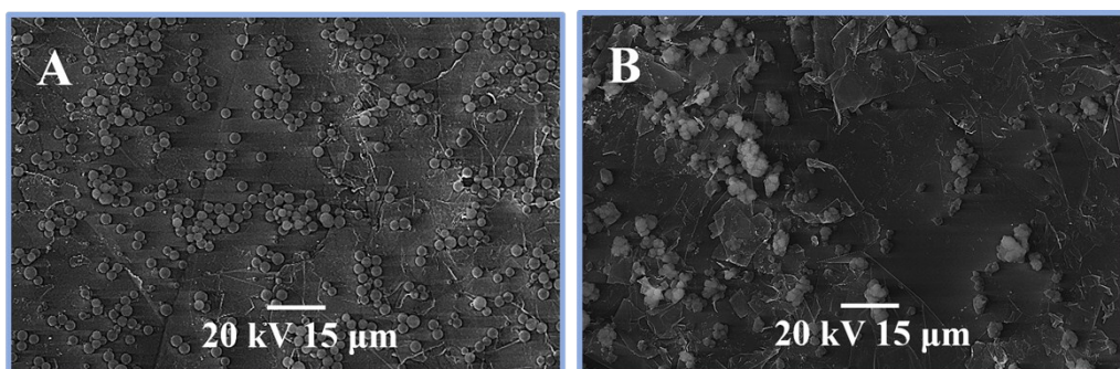
Fig. S1 SEM images of surface of MIPMSs/CPE (A) and MIPs/CPE (B)
