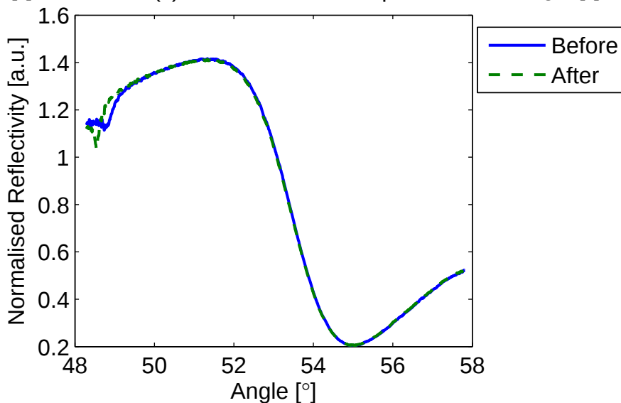
(c) SPR curves for soap
