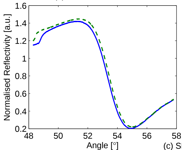
(a) SPR curves for bleach
