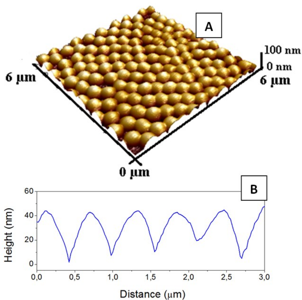
Fig. S1 – AFM topography (A) and surface profile of sandwich structure measured after the cooling/heating cycle in water.
