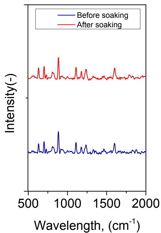
Fig. S2 – SERS spectra of pristine sandwich structure (PNIPAm response) before and after the cooling/heating cycle in water.
