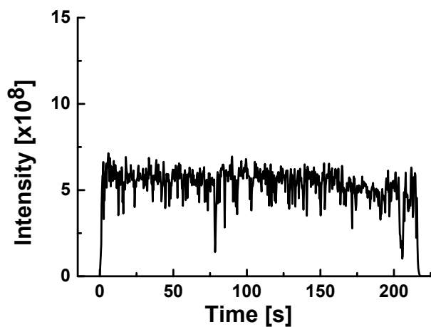
Fig. S-2 Example of the stability of the ion current obtained by using the thiol-ene \mu PESI chip. Extracted ion profile of protonated verapamil [M+H]^+ at m/z 455.2 \pm 0.3 . Injection volume of 3 \mu L (verapamil 5 \mu M in 1% HCOOH).
