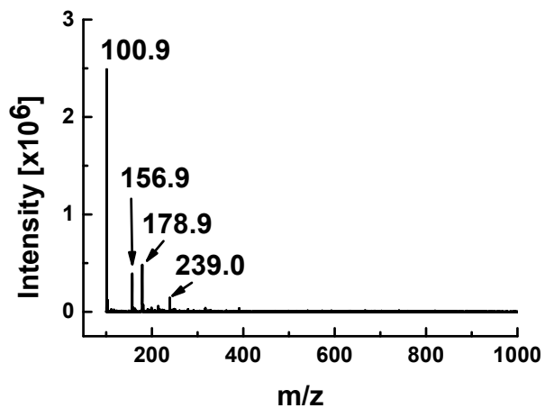
Fig. S-1 Background mass spectrum (50:49:1 MeOH:H 2 O:HCOOH).
