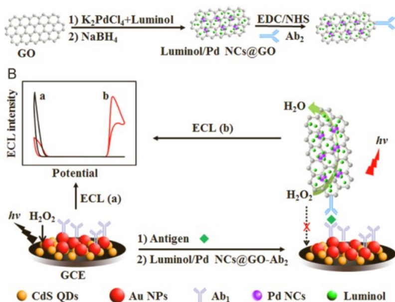
Reference 60. Scheme 1. Schematic illustration of (A) the synthesis of luminol/Pd NCs@GO-Ab 2 probe, (B) ratiometric ECL approach regulated by electrocatalysis of Pd NCs for highly sensitive detection of CEA.
