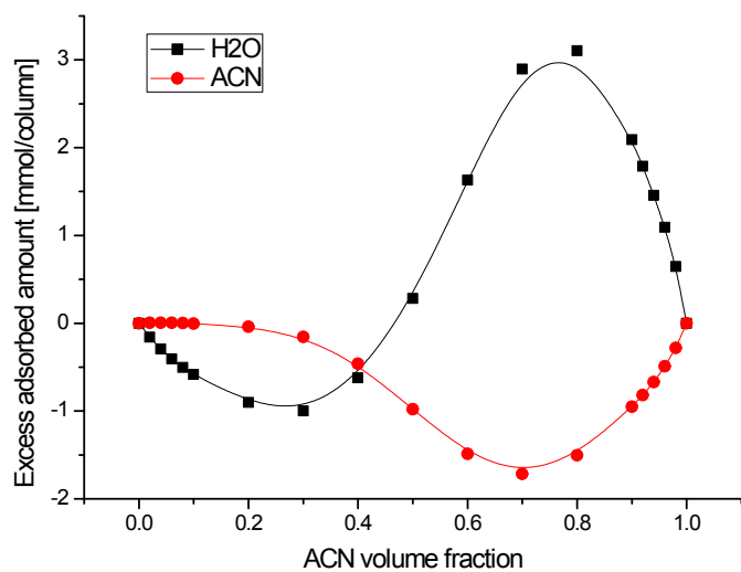
Figure S1 Excess adsorption isotherm of ACN and water on Amino-bonded stationary phase (synthesized on the same silica gel Kromasil 100A), column dimension 125×4.6 mm
