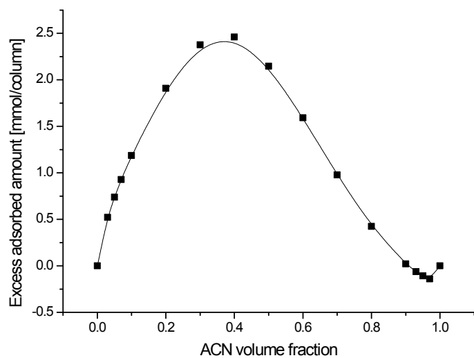
Figure S2 Excess adsorption isotherm of ACN on C18 stationary phase (synthesized on the same silica gel Kromasil 100A), column dimension 125×4.6 mm.
