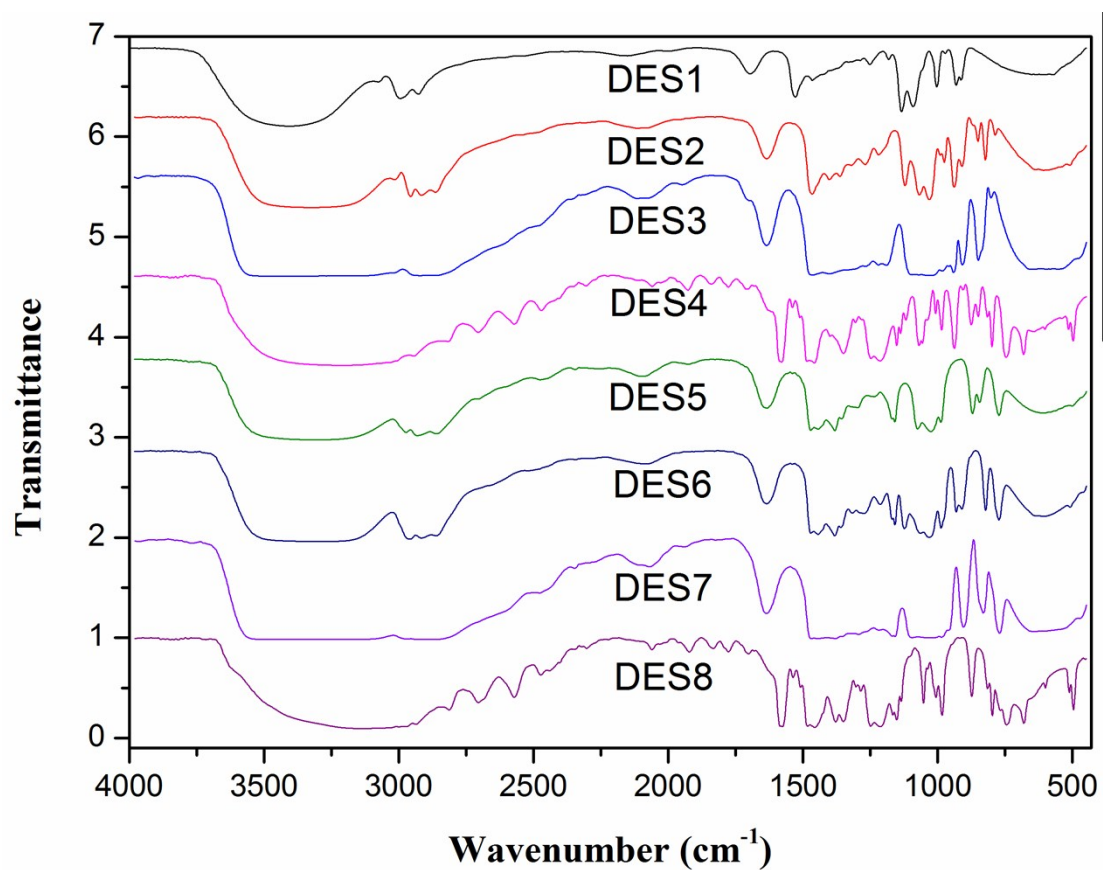
Fig. S1 FT-IR spectra of synthesized DESs
