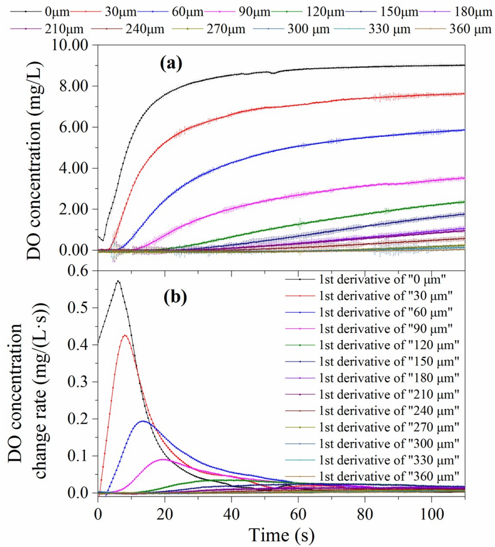
Fig. S2 (a) Oxygen-infuse processes in the inactive biofilm; (b) First-order derivatives of the DO concentrations in the inactive biofilm
