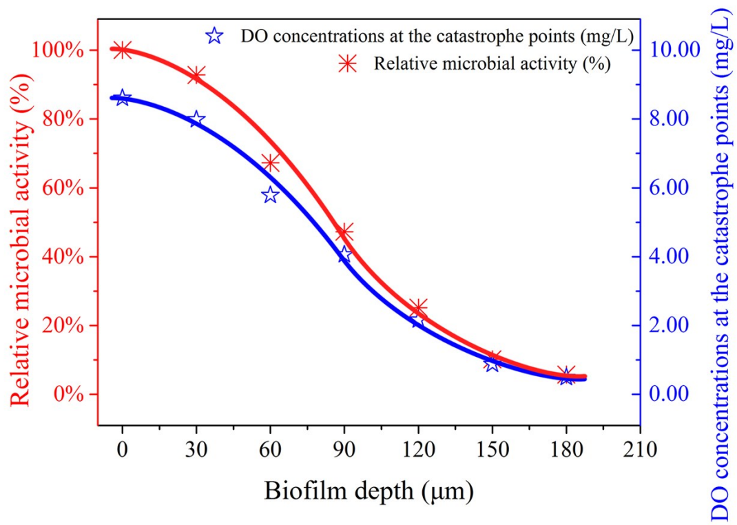
Fig. S3 DO concentrations at the catastrophe points and relative microbial oxygen metabolic activity microdistribution inside the active biofilm
