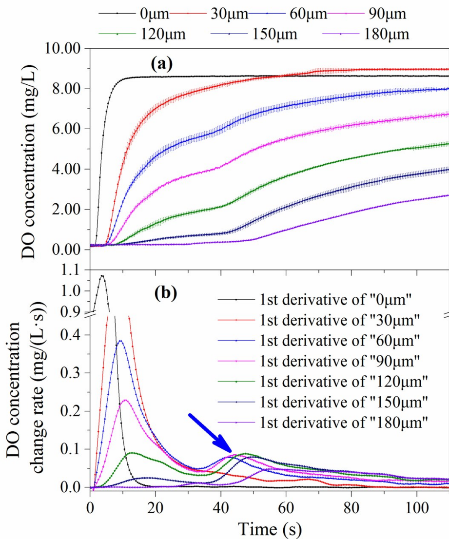
Fig. S1 (a) Oxygen-infuse processes in the active biofilm; (b) First-order derivatives of the DO concentrations in the active biofilm
