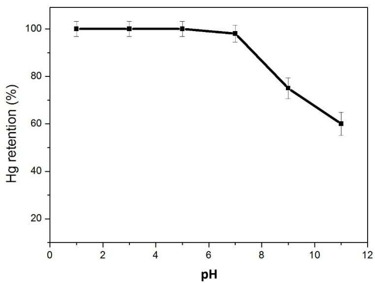
Fig. 3S. Influence of pH on the retention of Hg onto the IL-GO hybrid nanomaterial. Other conditions were as indicated in Table 1.
