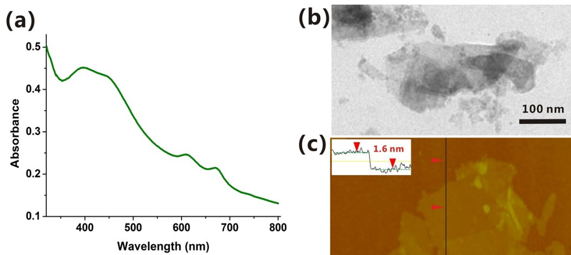
Fig. S1 (a) Typical UV-visible adsorption spectrum of the MoS 2 nanosheets. (b) TEM image of the MoS 2 nanosheets. (c) AFM and height profile (inset) images of the MoS 2 nanosheets.
