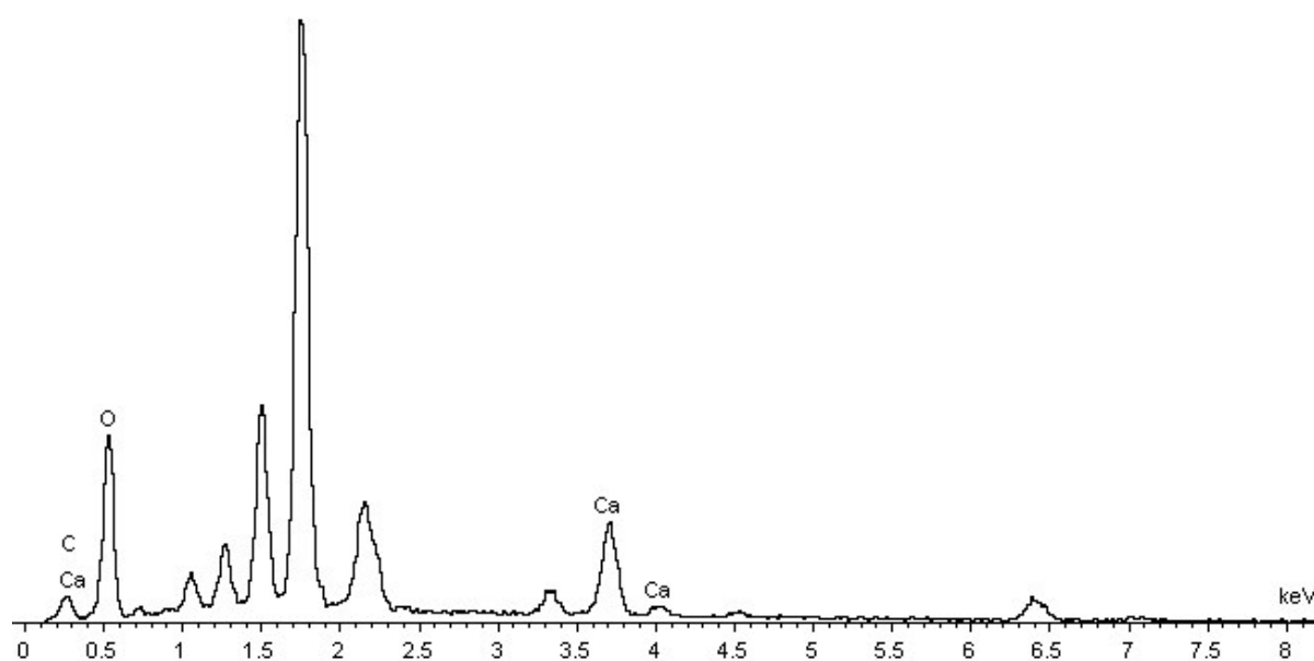
Fig. S1. The EDS image of nano- \text{CaCO}_3 .
