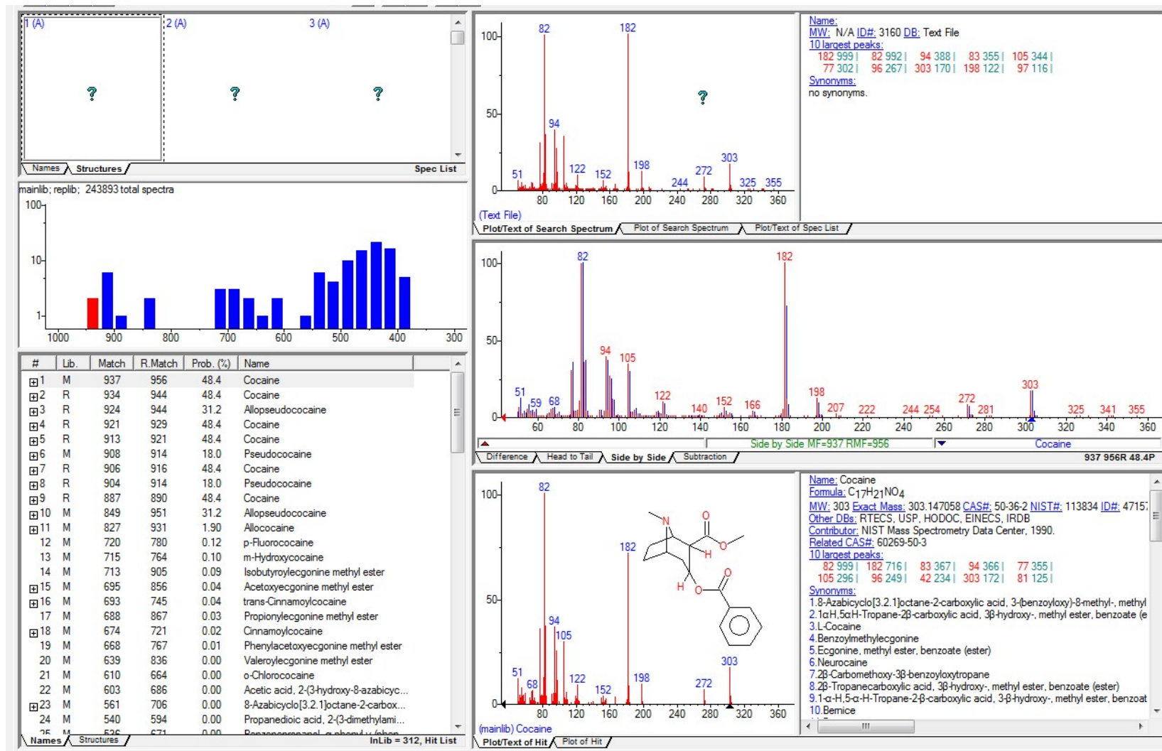
Figure 3S. GC-MS library containing the mass spectrum for cocaine.
